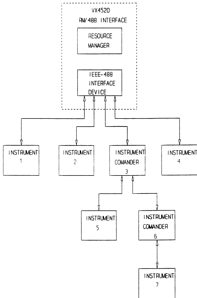
Figure 3: Typical System Hierarchy
